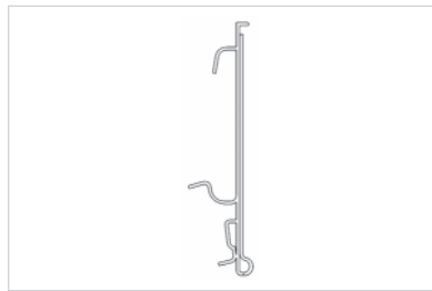
Clip-on ticket strip for Tegometall shelves with 5 mm overhang and with admission to make double profiles.
