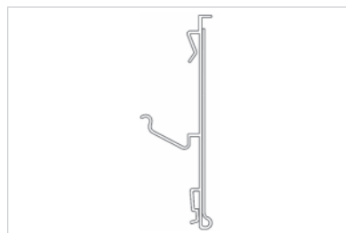
Clip-on ticket strip for Linde shelves with 5 mm overhang and with admission to make double profiles
